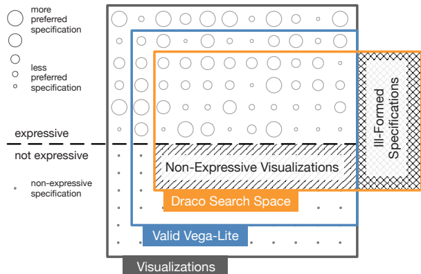
Fig. 3. Illustration of the design space in Draco. The set of valid Vega-Lite specifications is a subset of all possible visualizations, and Draco’s design space overlaps with that subset. Given a preference model, expressive visualizations are ranked according to their preference scores in the model. Draco eliminates ill-formed or non-expressive specifications using hard constraints and encodes preferences using soft constraints.
